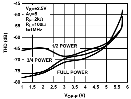
FIGURE 32. DIFFERENTIAL TOTAL HARMONIC DISTORTION vs DIFFERENTIAL OUTPUT VOLTAGE
